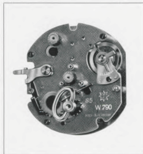
Platinen Plates - Platines - Platinas 50 x 43 mm = 2 x 1 3/4 inches
