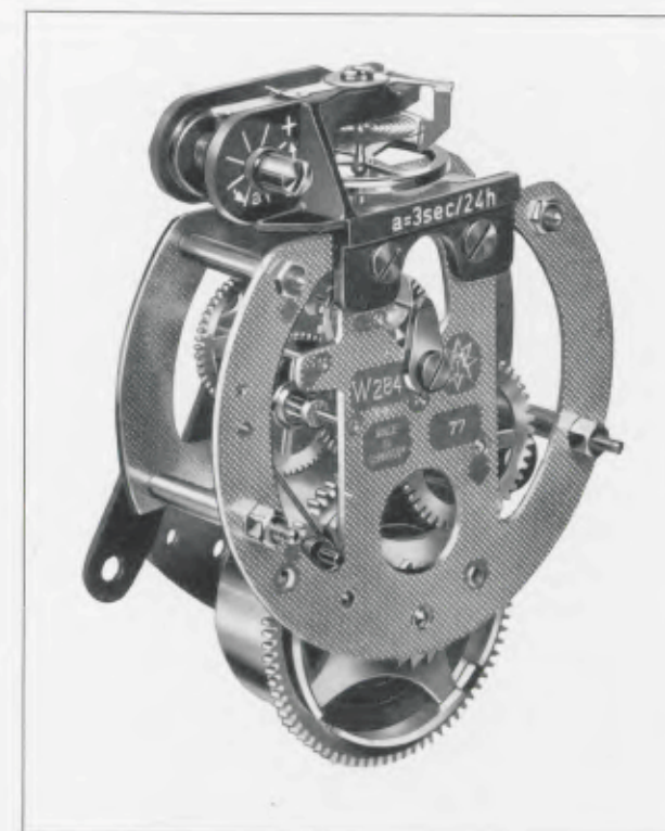
Platinen - Plates - Platines - Platinas 78 mm \varnothing - 3 1/16 inches
