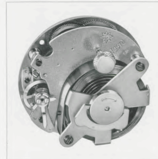
Platinen – Plates – Platines – Platinas 42 mm = 1 21 / 32 inches
