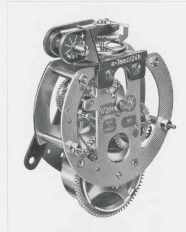
Platinen - Plates - Platinas - Platinas 78 mm \varnothing = 3 1/16 inches
