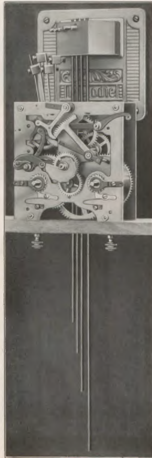
The 4 hammers strike simultaneously on the 4 rods.
