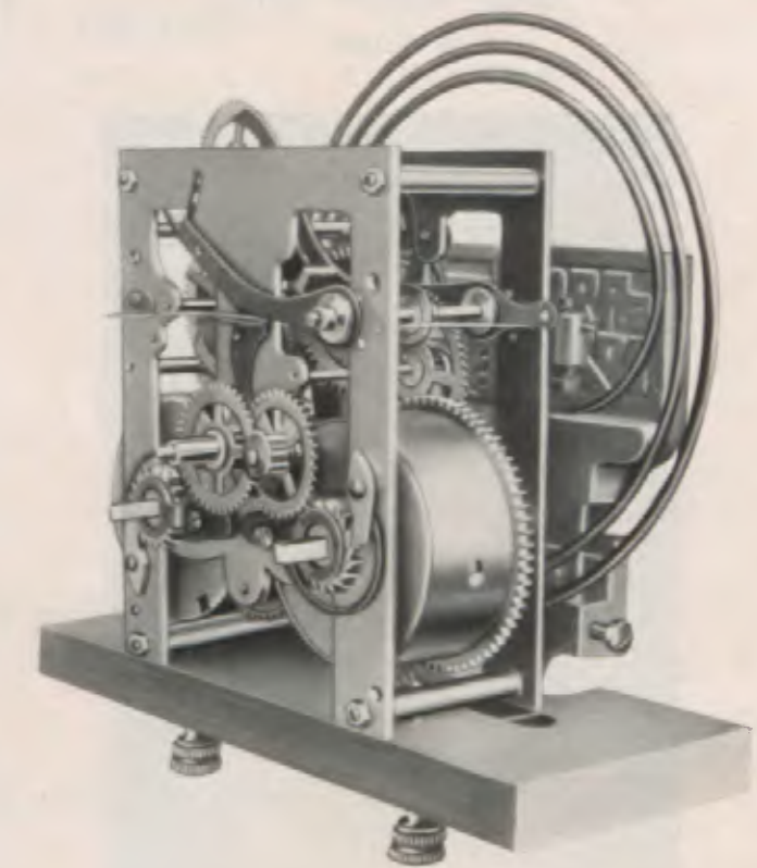
Movement No. 74 with "Kaiser"-Gong No. 139.
