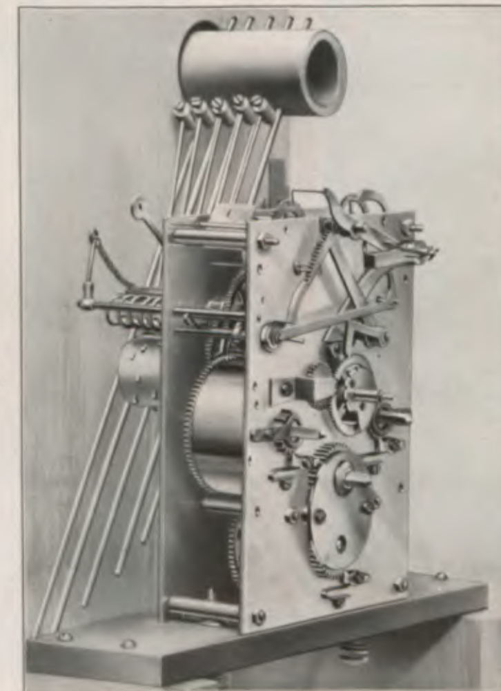
Movement No. 103 with Westminster Chime (5 rods).
